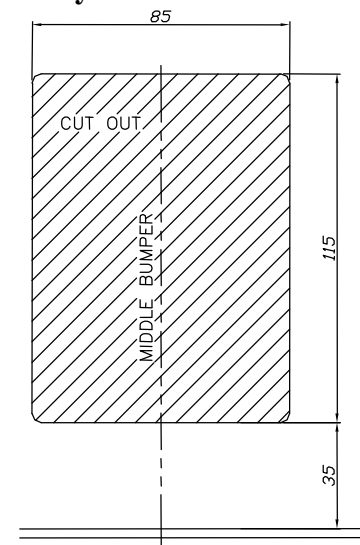
UNDERSIDE BUMPER
