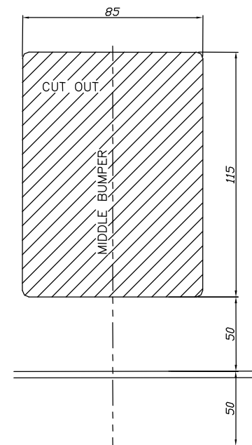
UNDERSIDE BUMPER
